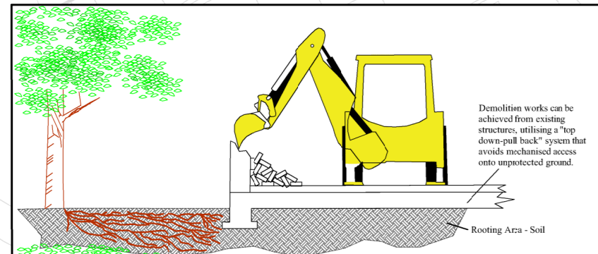
Examples of Ground Protection Systems
