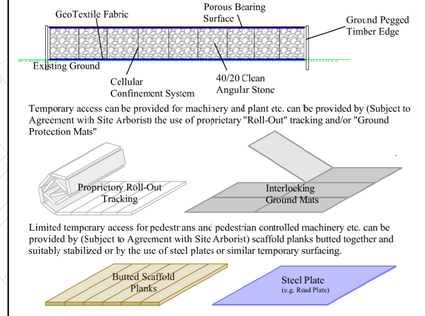
Examples of Ground Protection Systems
