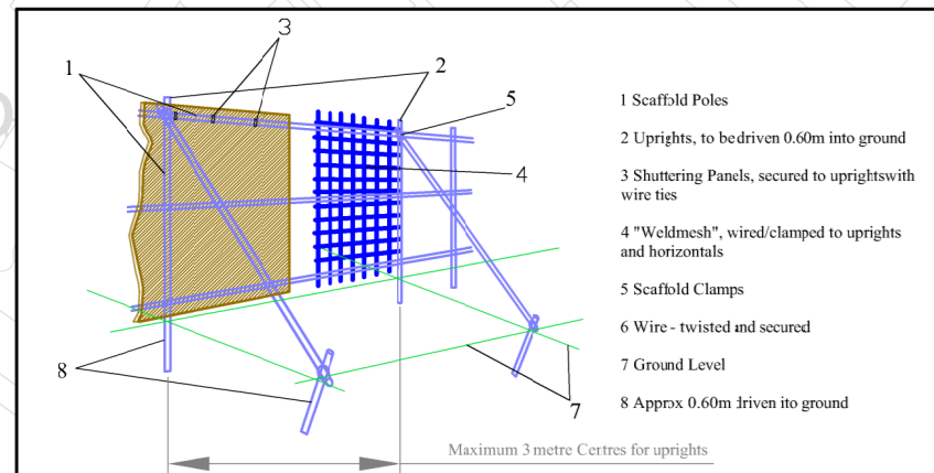
Example of Construction Methodology for "Construction Exclusion Fencing".
